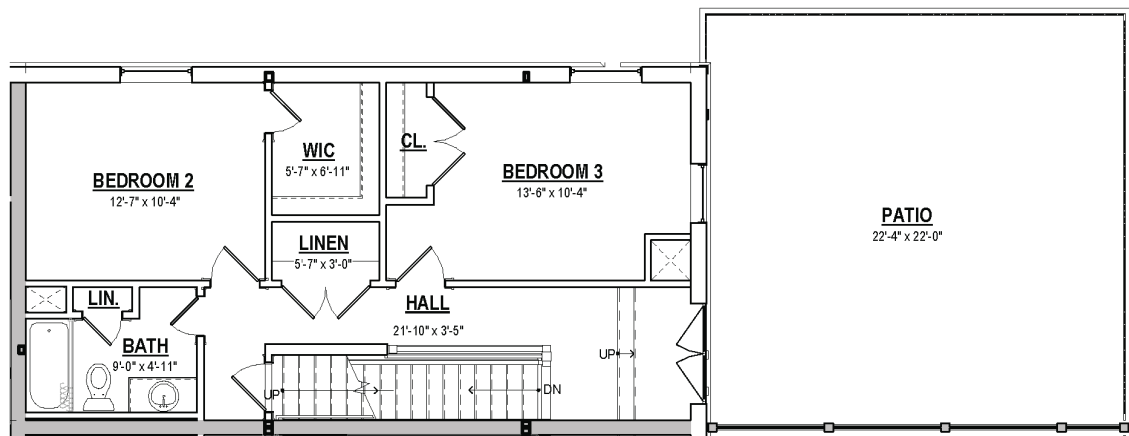
Second Floor
